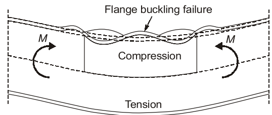
Fig. Local flange buckling failure
