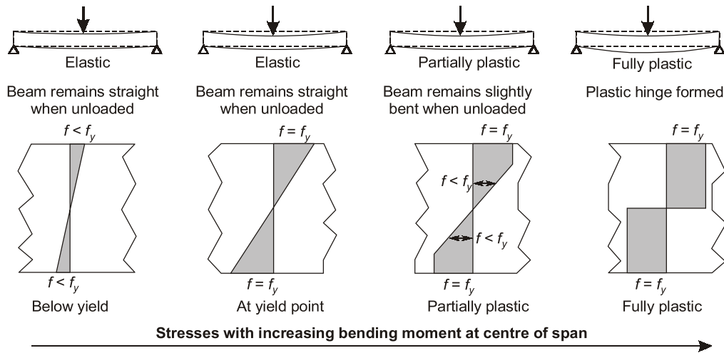
Fig. Various stages of beam bending failure
